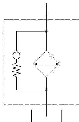
Schema idraulico Hydraulic circuit
